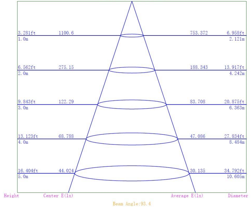
Illuminance-Distance Curve
