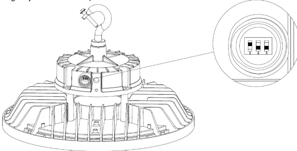
Default Wattage: 150W LOC-ELHB-MW(80/100/150)50KD-LV
