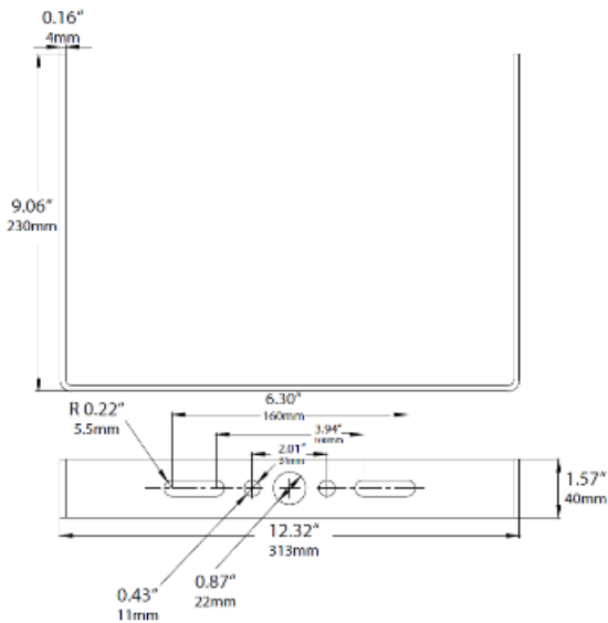
U-Bracket for 75W – 150W
