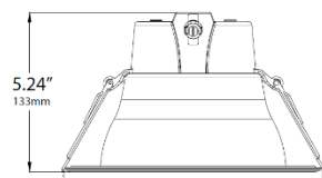
6" model
